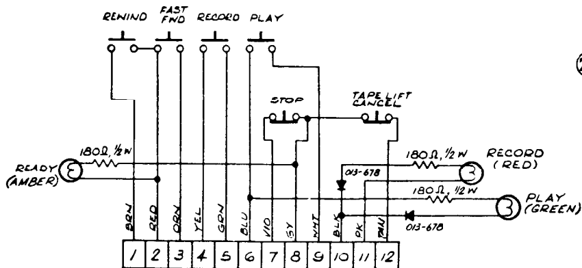
Assembly No. 4010080, Remote Control Assembly
