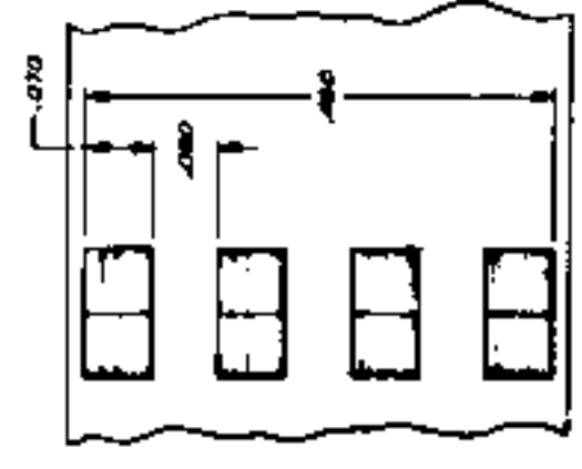
.070 TRACKS ON .80 CENTERS 6 TRACK 1/2" TAPE (.500/.496)
